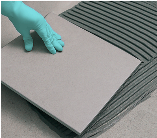
3. Tile Fixing
